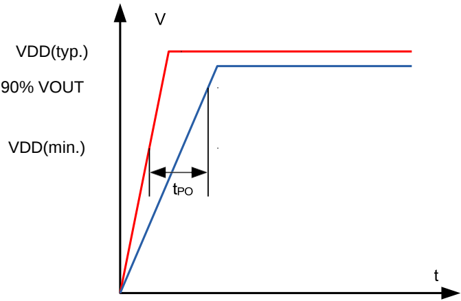
Figure 1. Power-On Time
