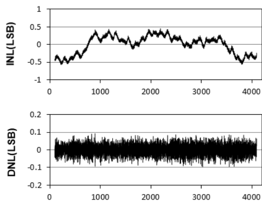
INL and DNL vs. Digital Input Code (125°C TPC112S1)
