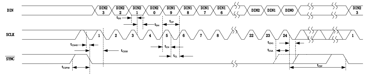
Figure 3. 24-Bit Serial-Interface Timing Diagram (TPC116S1)
