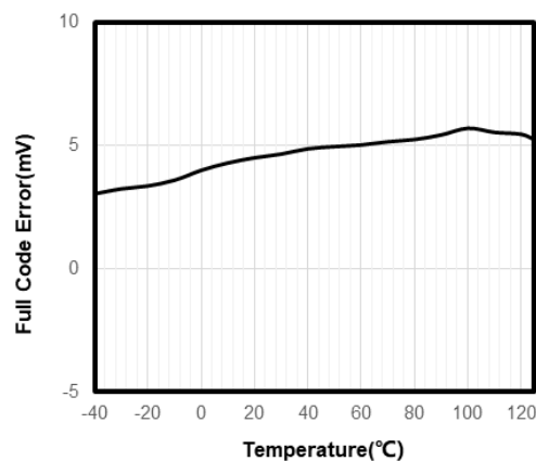
Full-Scale Error vs. Temperature (TPC112S1)
