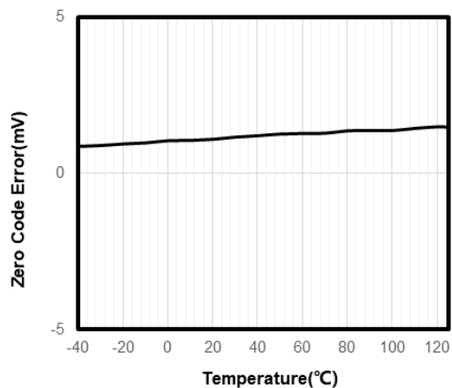
Zero-Scale Error vs. Temperature (TPC112S1)
