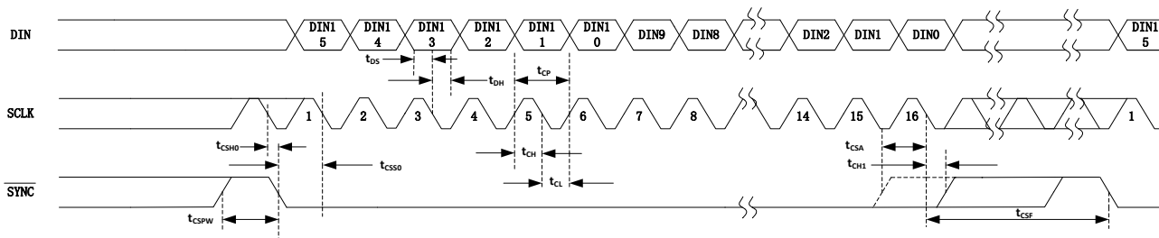
Figure 2. 16-Bit Serial-Interface Timing Diagram (TPC114S1)
