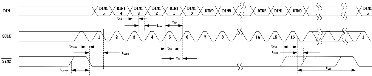
Figure 1. 16-Bit Serial-Interface Timing Diagram (TPC112S1)
