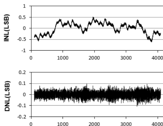
INL and DNL vs. Digital Input Code (25°C TPC112S1)
