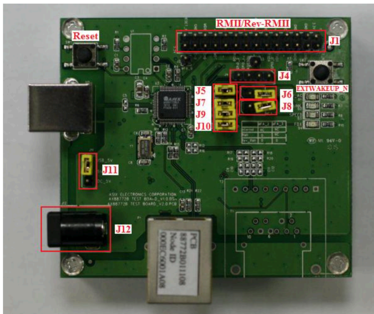
Figure 8. AX88772C USB to 100Base-TX Ethernet (with RMII) Demo Board
