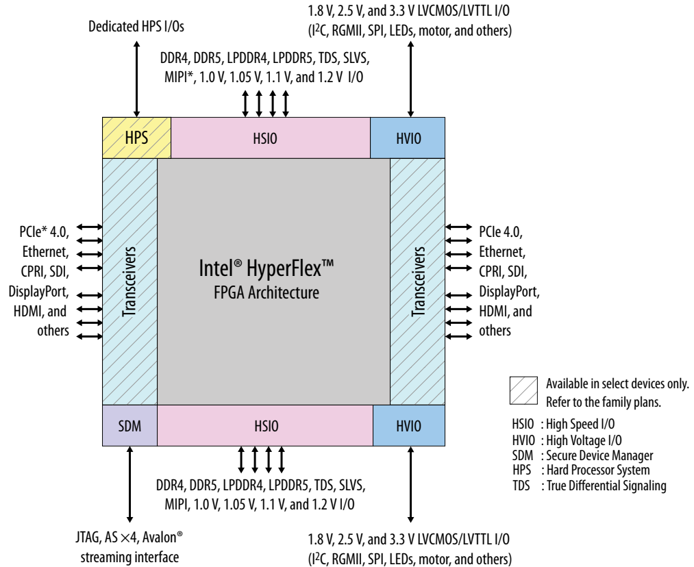
Figure 1. Agilex 5 FPGAs and SoCs Block Diagram
