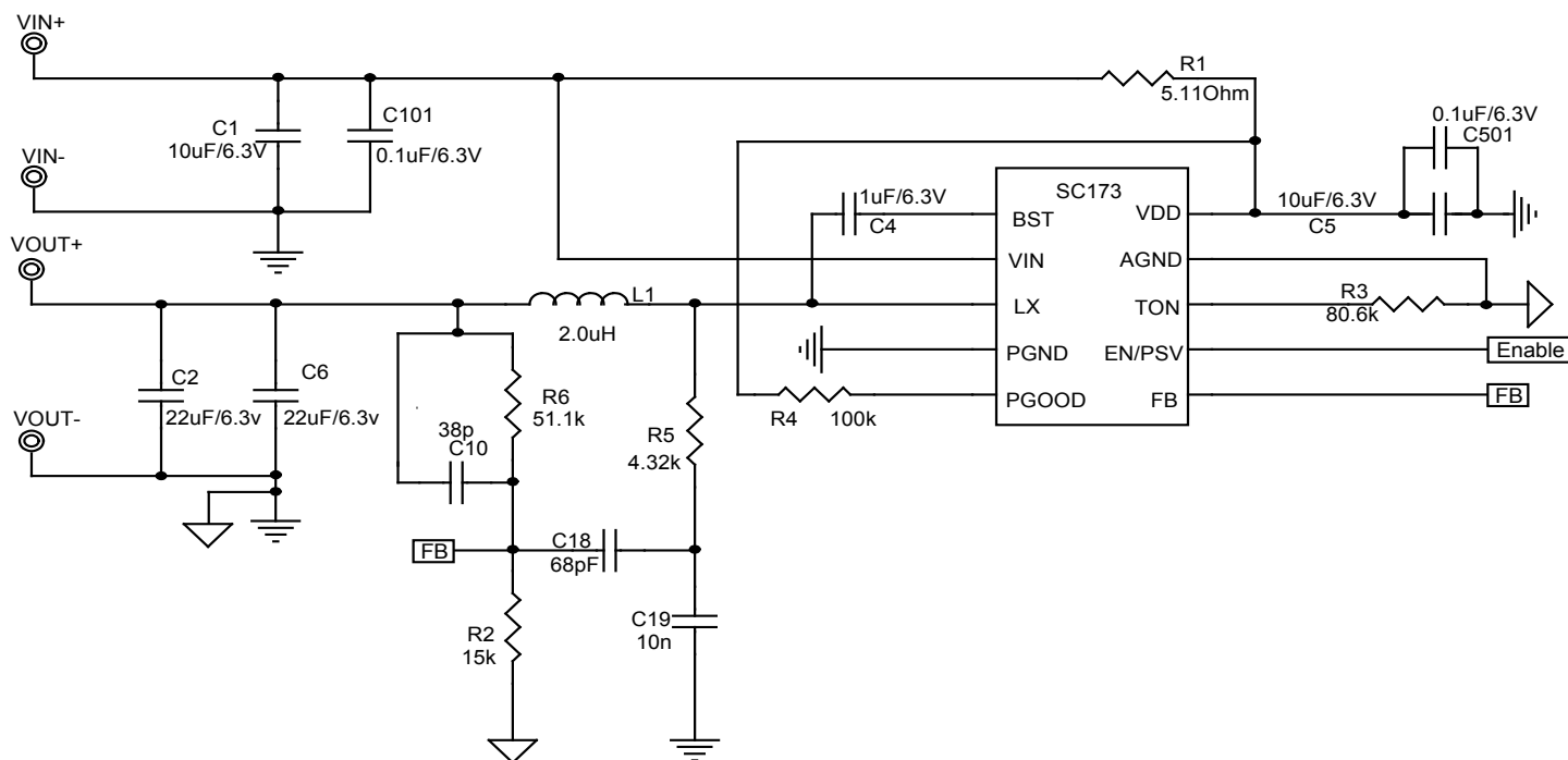
Application Circuit: Buck Converter with 3.3V out and 0 to 3A load current (Vin=5V)
