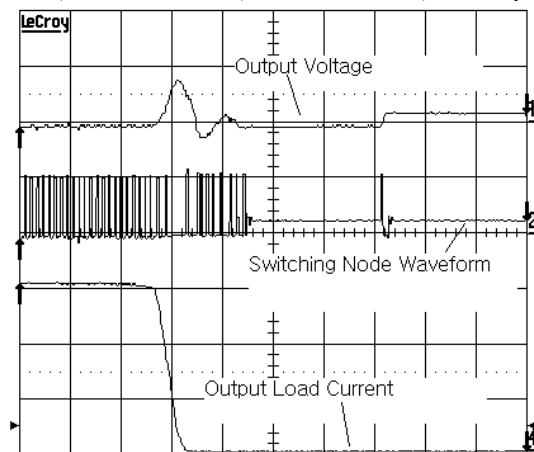
Load Transient Test ( V_{IN}=5V , V_{OUT}=1.2V , I_{OUT}= 3A to 0A , PSAVE Mode Enabled, L_{OUT}=1.3\mu H , C_{OUT}=2\times 22\mu F , Channel 1: 100mV/Div,Channel 2:5V/Div,Channel 4:1A/Div, Time:20 \mu s /Div)
