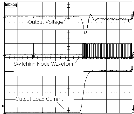
Load Transient Test ( V_{IN}=5V , V_{OUT}=1.2V , I_{OUT}= 0A to 3A , PSAVE Mode Enabled, L_{OUT}=1.3\mu H , C_{OUT}=2\times 22\mu F , Channel 1: 50mV/Div, Channel 2:5V/Div,Channel 4:1A/Div,Time:10 \mu s /Div)
