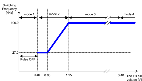
Figure 5B. Switching Frequency vs the FB Pin Voltage (BM2P104H-Z)
