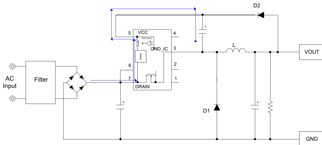
Figure 5. Start circuit
