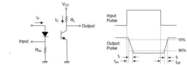
Fig.10 Switching Time Test Circuit & Waveforms
