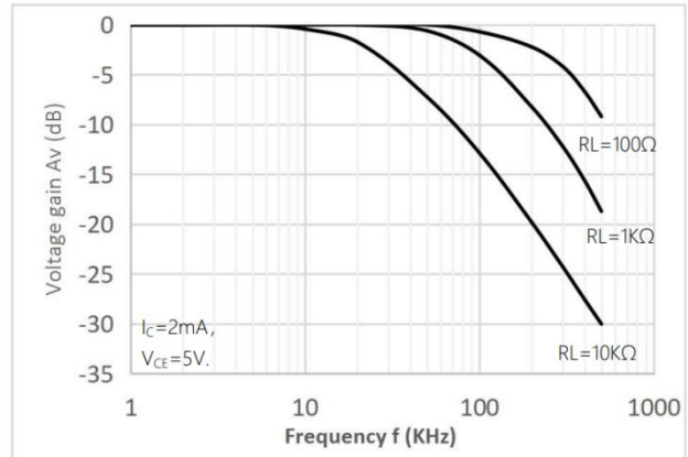
Fig.8 Frequency Response
