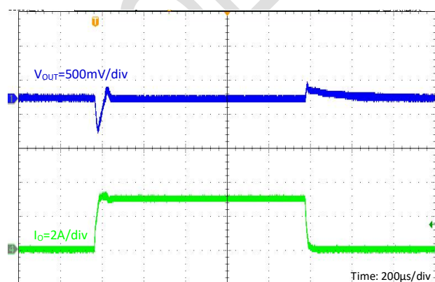
Load Transient
