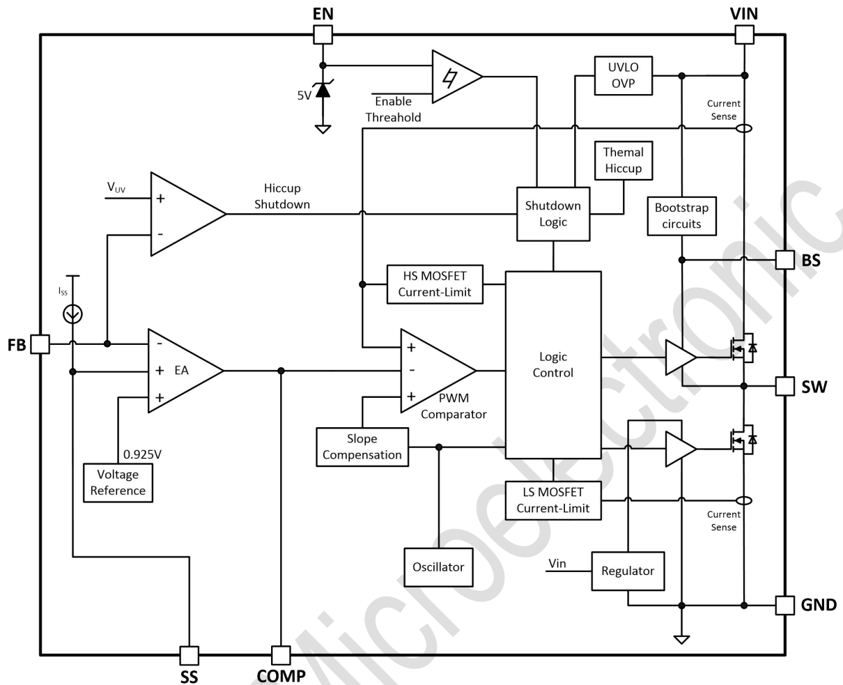
Figure 2. TMI3344 Block Diagram
