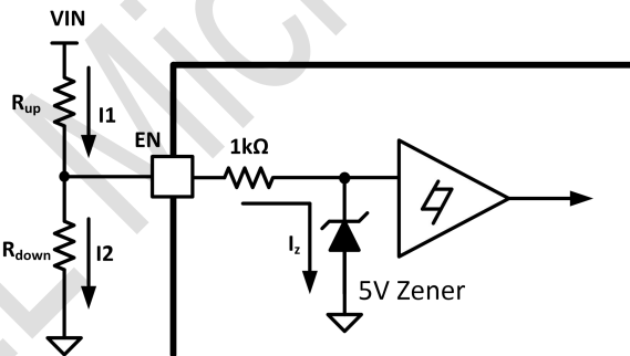
Figure 3. EN pin external connection
