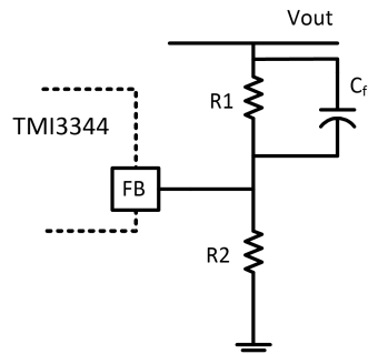
Figure 4. Output Voltage Setting
