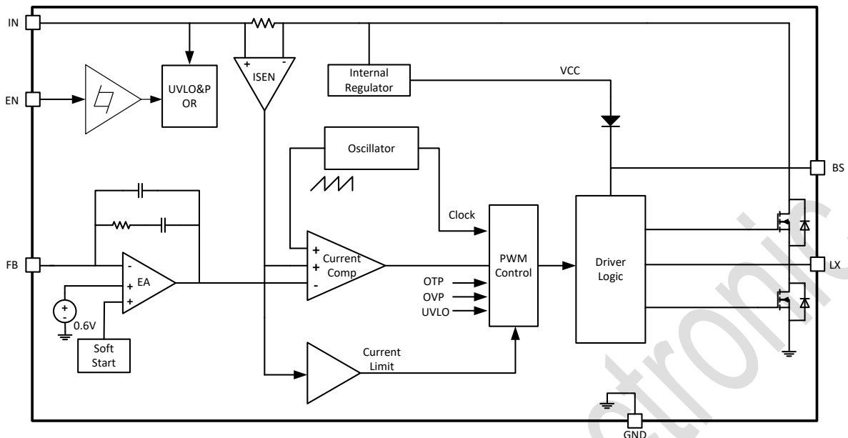
Figure 2. TMI3280 Block Diagram
