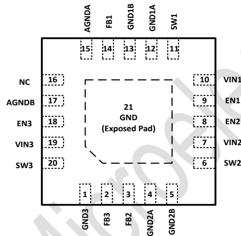
QFN3x3-20L (Top View)
