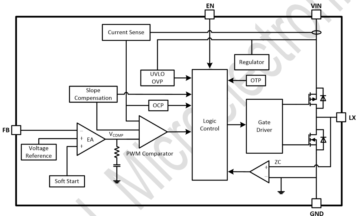
Figure 2. STI34061 Block Diagram
