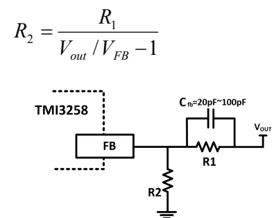
Figure 2. Feedback Network
