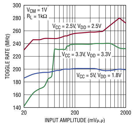
Toggle Rate vs Input Amplitude, LTC6752-3
