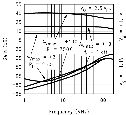
Feed-Through Isolation
