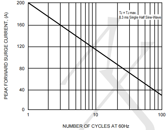
FIG. 2 - MAXIMUM NON-REPETITIVE
