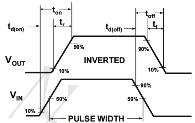
Figure 2: Switching Waveforms
