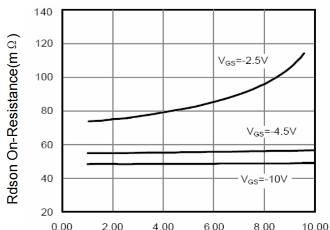
Figure 6 Drain-Source On-Resistance
