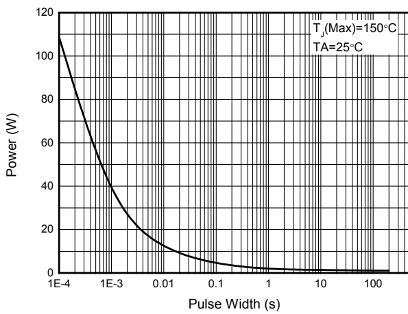
Figure 9: Single Pulse Power Rating Junction-to-Ambient (Note E)
