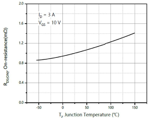
Figure 6. Normalized On-Resistance
