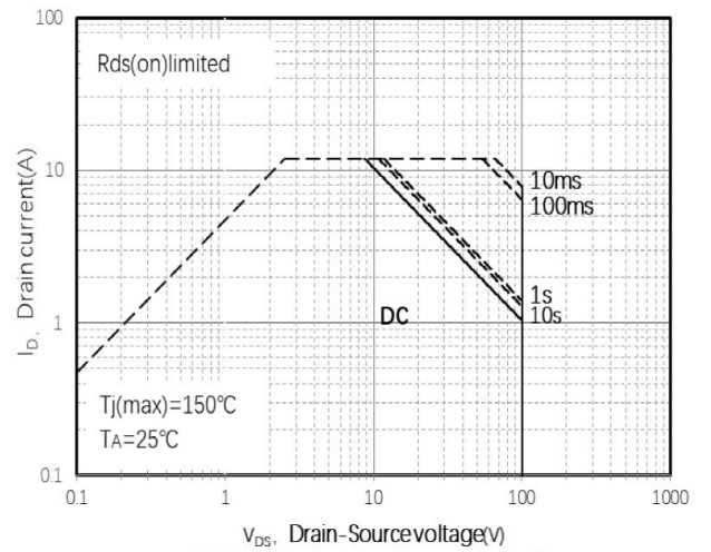
Figure8.Safe Operation Area
