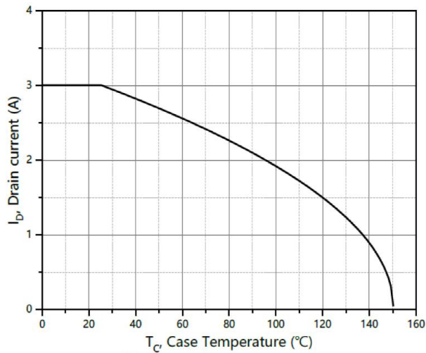
Figure7. Drain current
