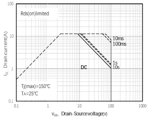
Figure8.Safe Operation Area
