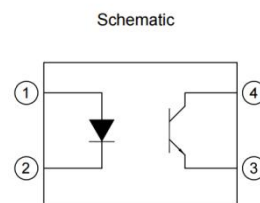
Pin Configuration 1 Anode 2 Cathode 3 Emitter 4 Collector
