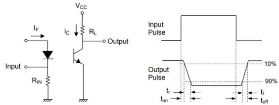
Fig.10 Switching Time Test Circuit & Waveforms
