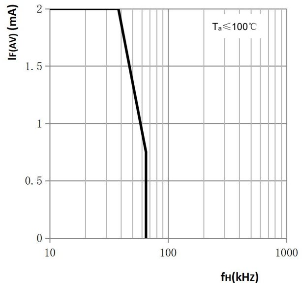
Figure 4. I_{F(AV)} - f_H Curve
