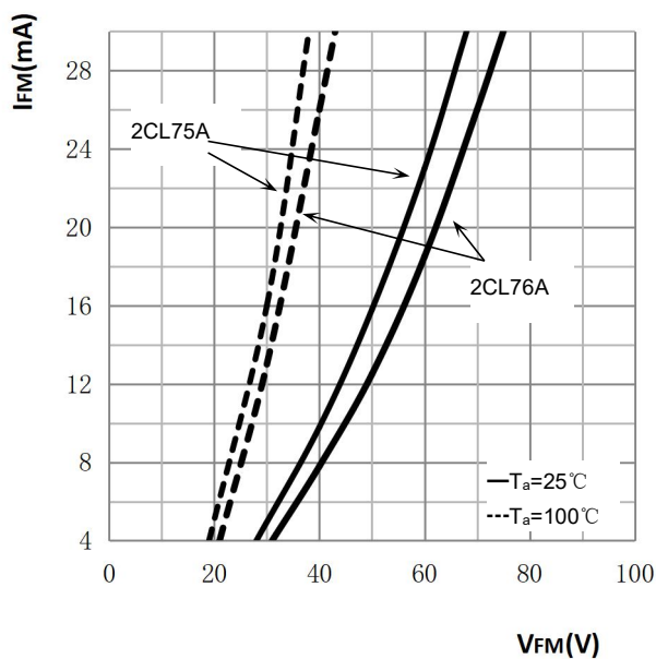
Figure 1. Forward characteristics
