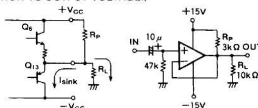
Fig. 7 (Explanation by dual power supply method)
