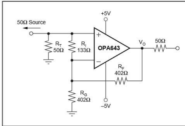
FIGURE 5. Broadband Low Gain Non-Inverting External Compensation.
