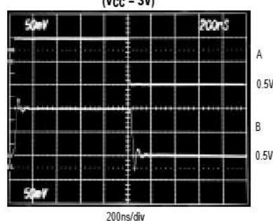
SMALL-SIGNAL TRANSIENT RESPONSE ( V_{CC} = 3V )
