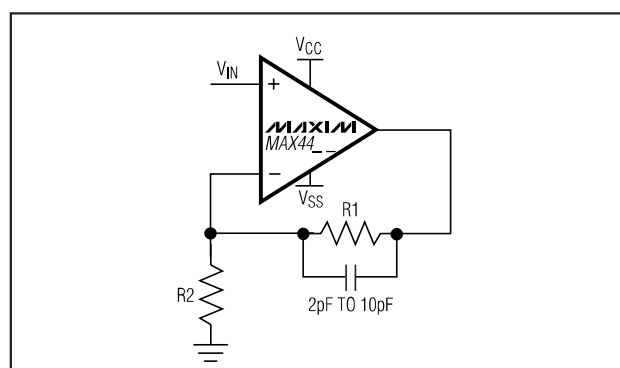
Figure 1. Compensation for Feedback Node Capacitance
