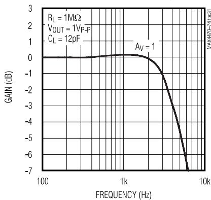
MAX4470/MAX4471/MAX4472 LARGE-SIGNAL GAIN vs. FREQUENCY
