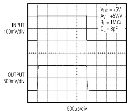
MAX4464/MAX4474 LARGE-SIGNAL STEP RESPONSE
