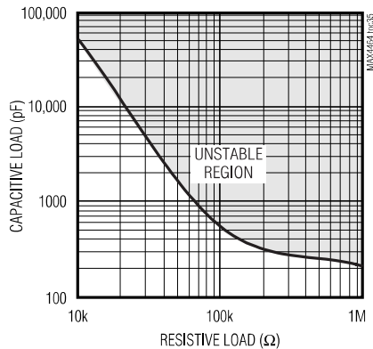
MAX4464/MAX4474 STABILITY vs. CAPACITIVE AND RESISTIVE LOADS
