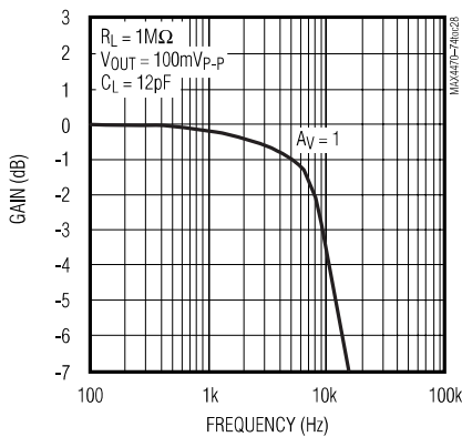
MAX4470/MAX4471/MAX4472 SMALL-SIGNAL GAIN vs. FREQUENCY
