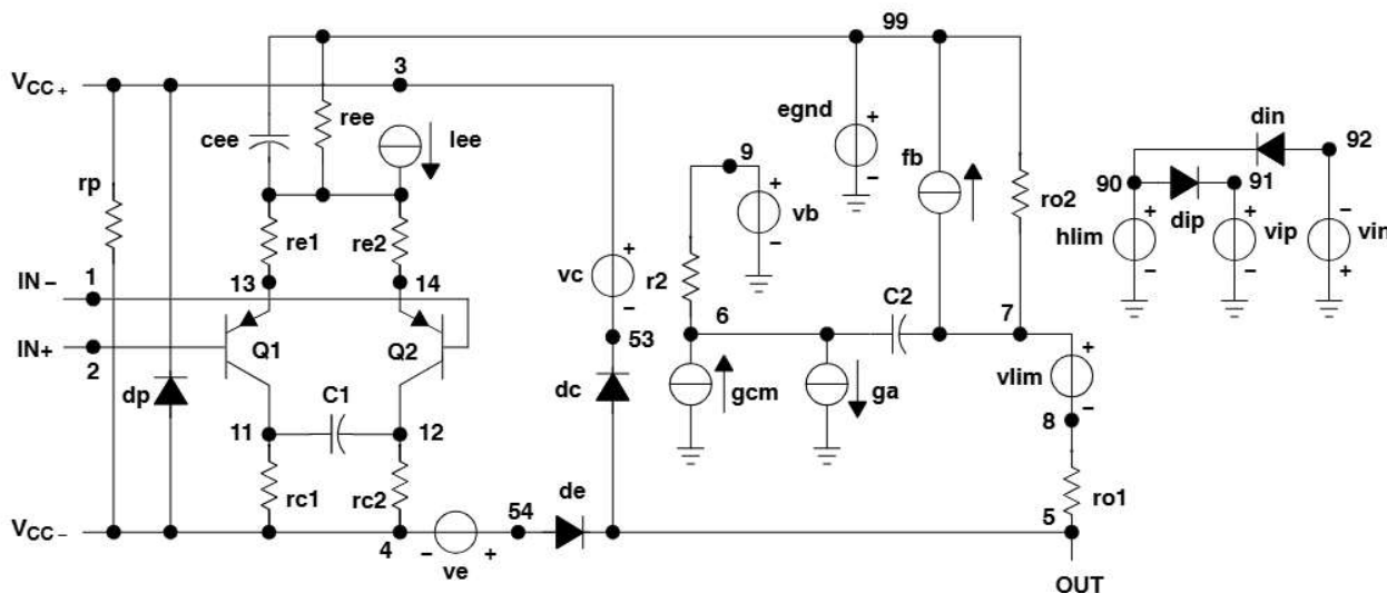
Figure 73. Boyle Subcircuit
