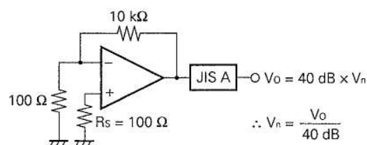
Fig. 3 Flat Noise Measurement Circuit (FLAT + JIS A)
