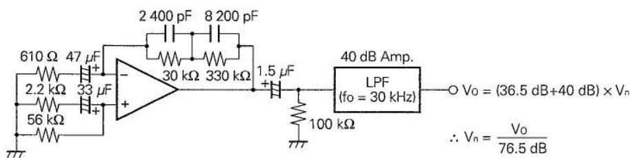
Fig. 2 Noise Measurement Circuit (RIAA)
