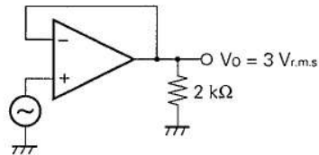
Fig. 1 Total Harmonic Distortion Measurement Circuit
