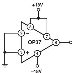
Figure 3. Burn-In Circuit
