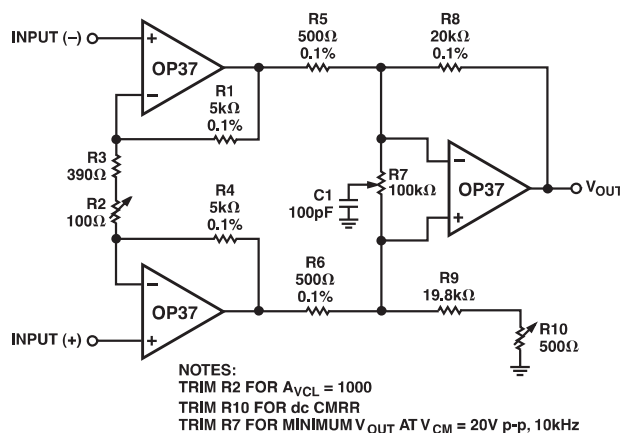
Figure 4a. Instrumentation Amplifier
