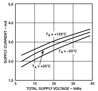
TPC 9. Supply Current vs. Supply Voltage
