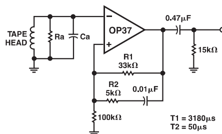
Figure 9. Tape-Head Preamplifier
