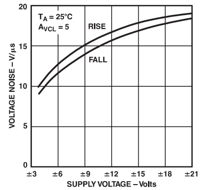
TPC 33. Slew Rate vs. Supply Voltage
