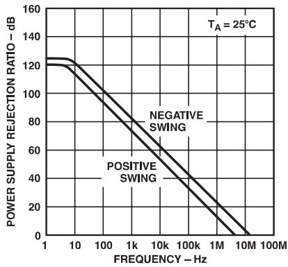
TPC 31. PSRR vs. Frequency
