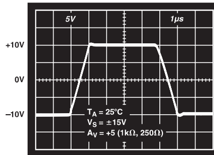
TPC 23. Large-Signal Transient Response
