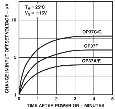
TPC 12. Warm Up Offset Voltage Drift of Six Representative Units
