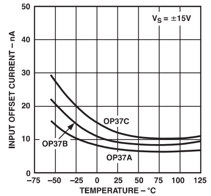
TPC 15. Input Offset Current vs. Temperature
