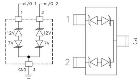
PIN Configuration
