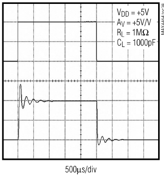
MAX4464/MAX4474 SMALL-SIGNAL STEP RESPONSE
