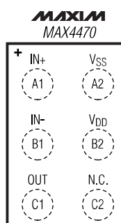
WLP BUMP SIDE DOWN
