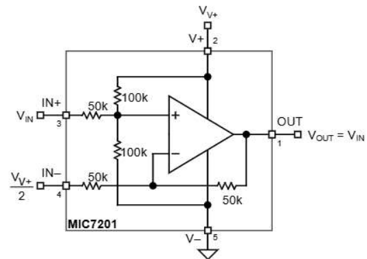
Figure 3. Voltage Follower
