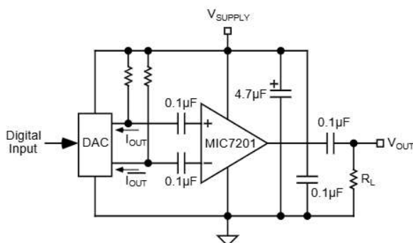
Figure 1. Audio DAC
