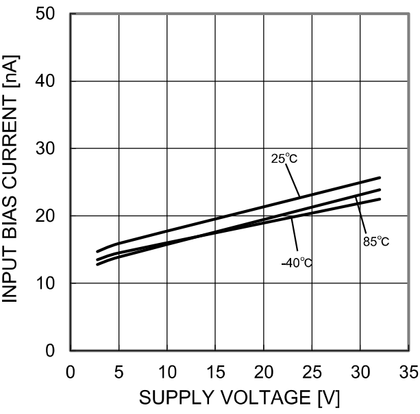
Figure 15. Input Bias Current - Supply Voltage ( V_{ICM}=0V , OUT=1.4V )
