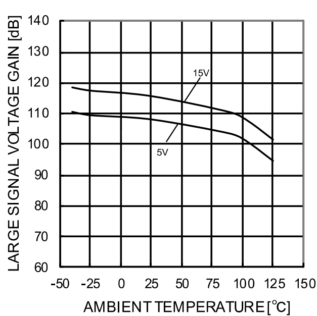
Figure 70. Large Signal Voltage Gain - Ambient Temperature (RL=2kΩ)
