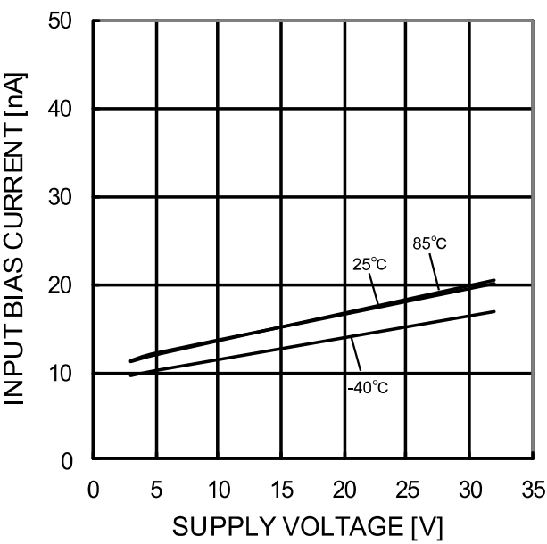
Figure 39. Input Bias Current - Supply Voltage ( V_{ICM}=0V , OUT=1.4V )
