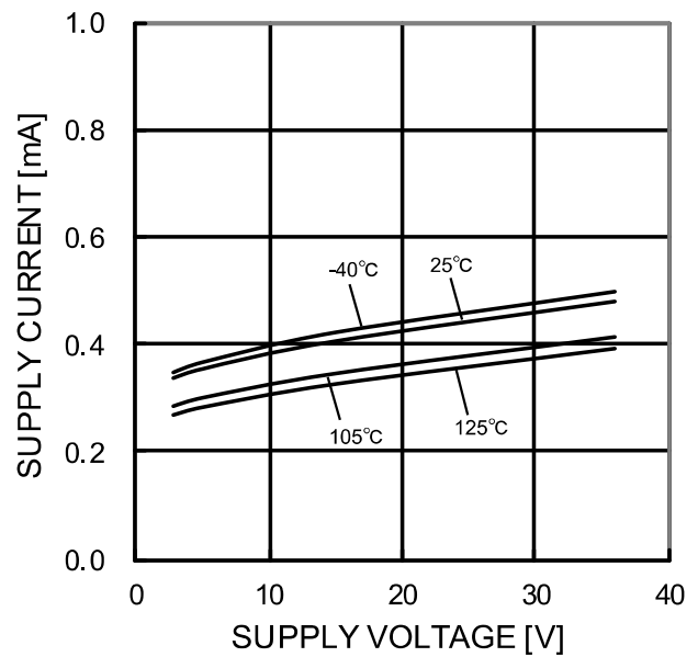
Figure 51. Supply Current- Supply Voltage
