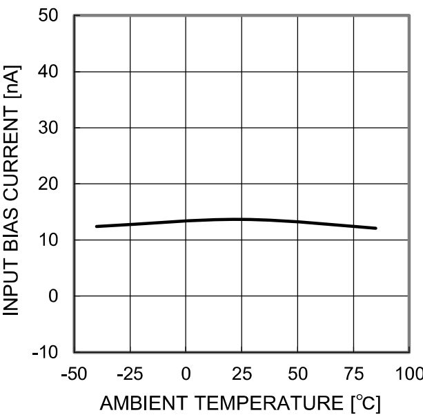
Figure 17. Input Bias Current - Ambient Temperature ( V_{CC}=30V , V_{ICM}=28V , OUT=1.4V )
