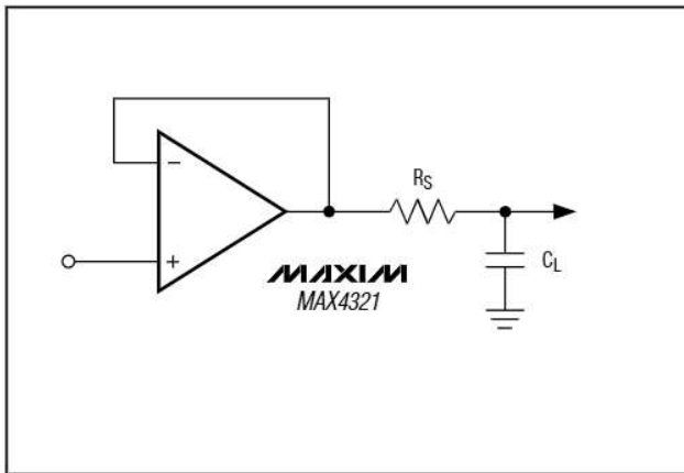
Figure 7. Capacitive-Load-Driving Circuit
