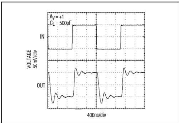
Figure 5. Small-Signal Transient Response with Capacitive Load
