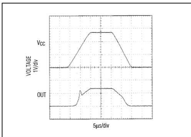
Figure 9. Power-Up Output Voltage
