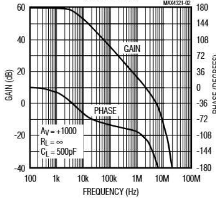
GAIN AND PHASE vs. FREQUENCY (WITH LOAD)
