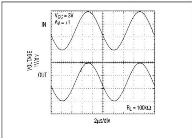
Figure 3. Rail-to-Rail Input /Output Voltage Range
