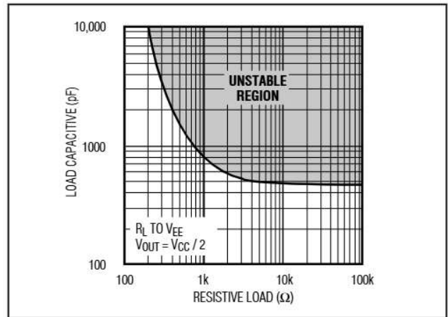
Figure 4. Capacitive-Load Stability
