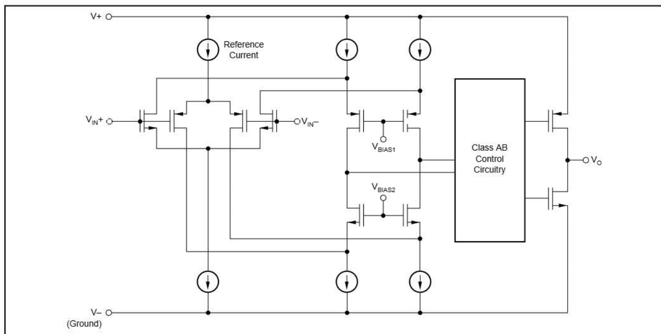
FIGURE 2. Simplified Schematic.
