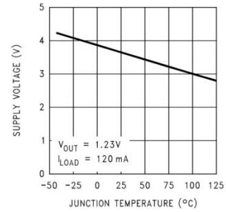
Minimum Operating Supply Voltage
