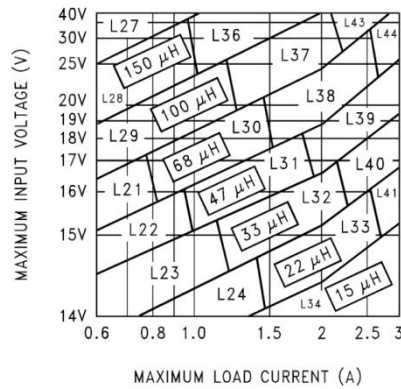
FIGURE 6. XH2596-12
