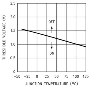
ON/OFF Threshold Voltage
