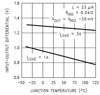
Dropout Voltage
