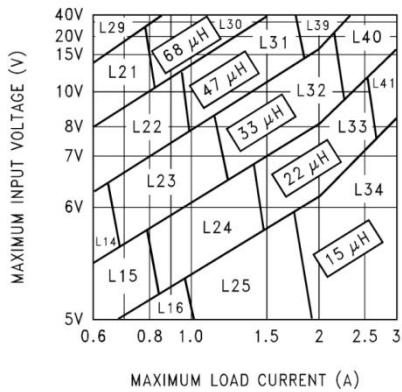
FIGURE 4. XH2596-3.3
