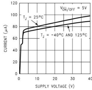
Shutdown Quiescent Current
