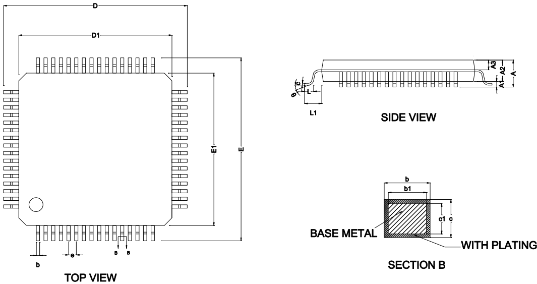
图 4-2 LKS32MC453RCT8/LKS32MC455RCT8/LKS32MC455LRCT8 封装图示
