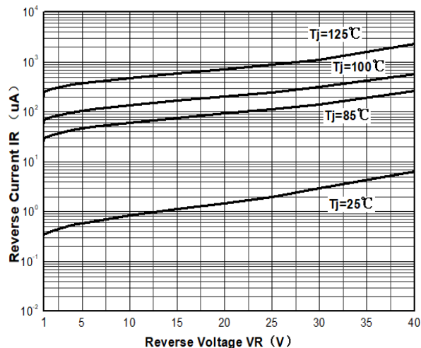
Reverse Characteristics
