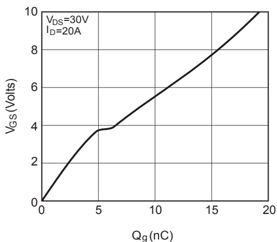
Gate-Charge Characteristics
