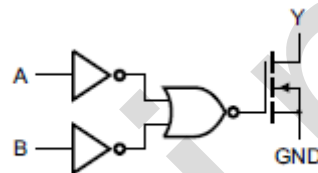
Figure 3. Logic diagram
