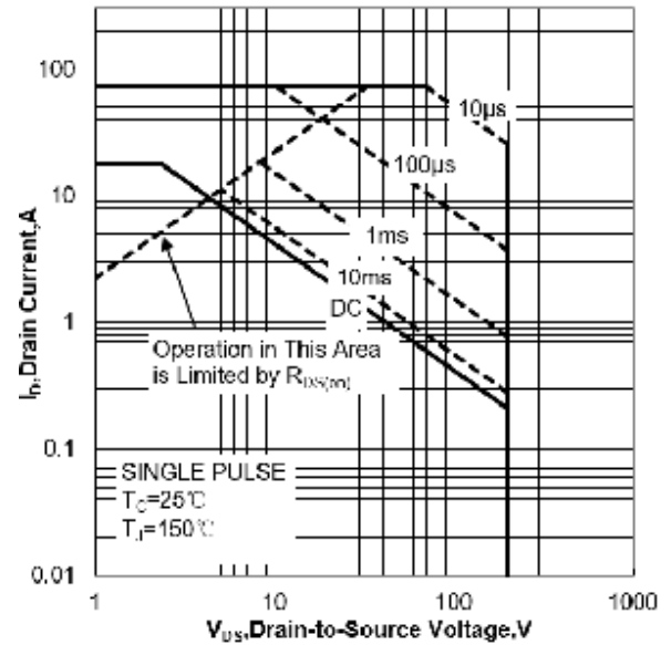
Figure 1b Safe Operating Area (FullPAK)
