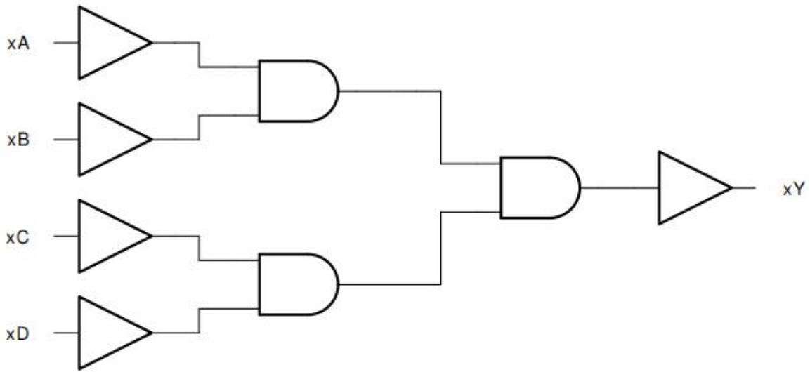
Figure 3.1: 74HC21 Logic Diagram
