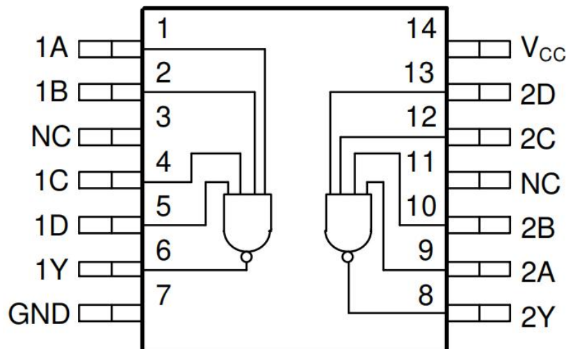
Figure 2.1: Top View
