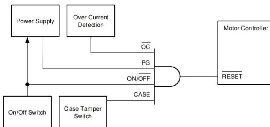
Figure 5.1: Typical application schematic
