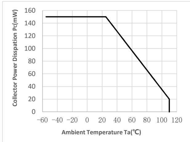
Fig.2 AllowaPCe collector power dissipation vs. Ambient Temperature (°C)
