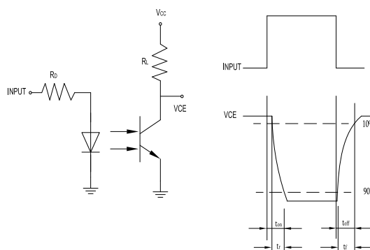
Fig.12 Switching Time Test Circuit & Waveforms
