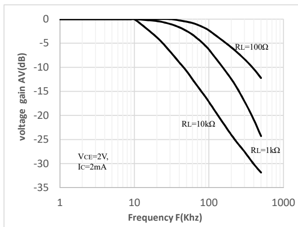
Fig.10 Frequency Response
