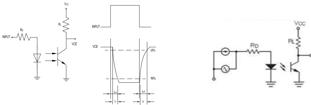
Fig.12 Switching Time Test Circuit & Waveforms
