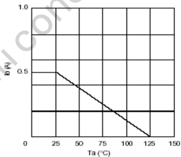
Fig.4 Derating curve
