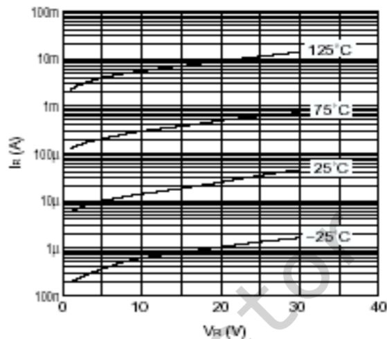
Fig.2 Reverse characteristics
