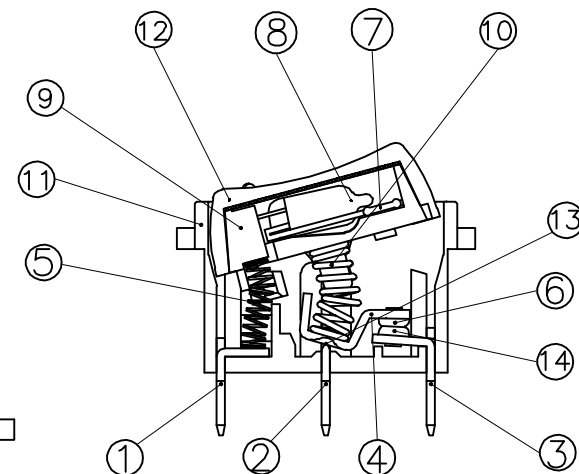
ASSEMBLE DRAWING
