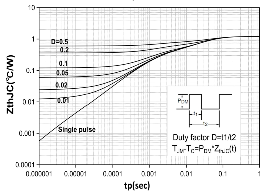
Transient Thermal Response Curve For TO-252
